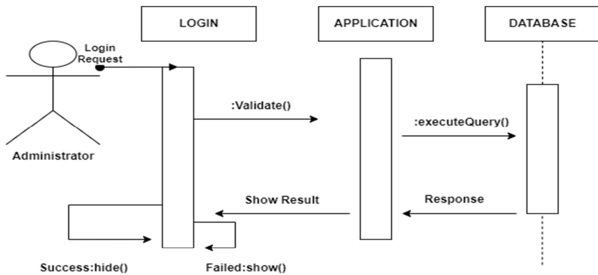
SEQUENCE DIAGRAM FOR ADMINISTRATOR
