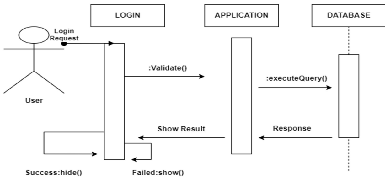
SEQUENCE DIAGRAM FOR USER
